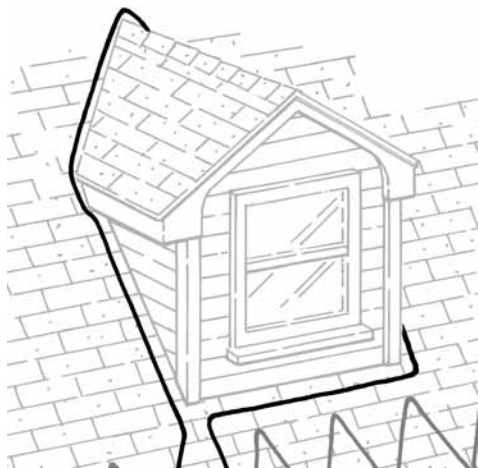
Figure 7. Cable pattern around a dormer
