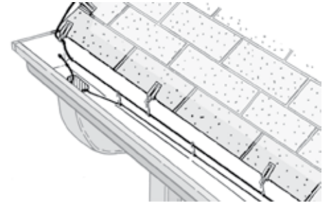
Figure 20b. Double run of cable in gutter-only applications (gutters without gutter spikes)
