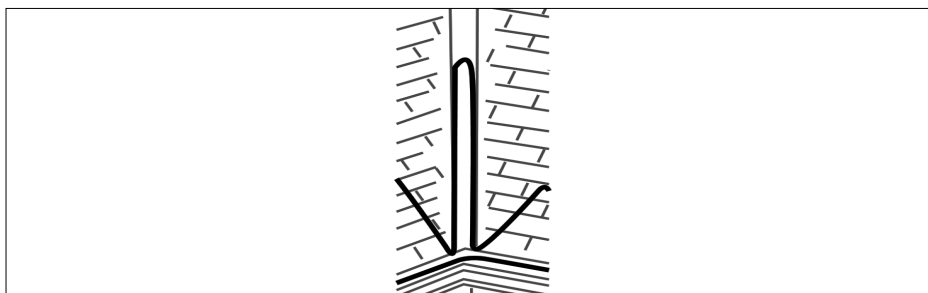
Figure 5. Configuration de la noue
