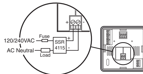
Figure 3.11 Control Output Wiring—V0
