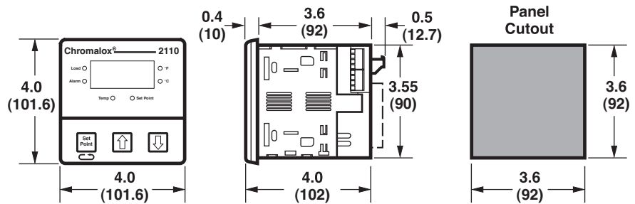
Figure 3.3 Mounting Dimensions
