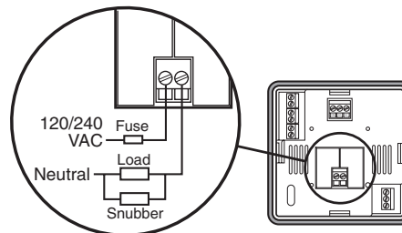
Figure 3.9 Control Output Wiring—R1 and S0
