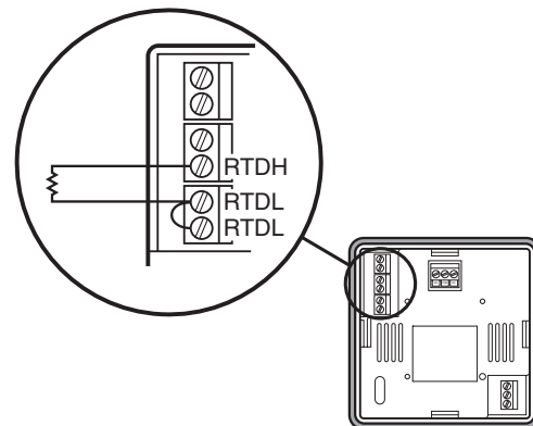
Figure 3.8 Two-Wire RTD Connections
