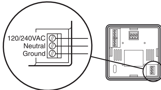
Figure 3.13 90-260 VAC Instrument Power Connections
