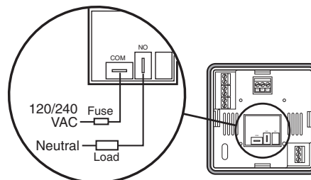
Figure 3.10 Control Output Wiring—R3
