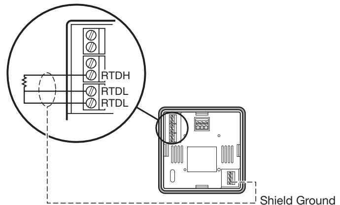
Figure 3.7 Three-Wire RTD Connections with Shield
